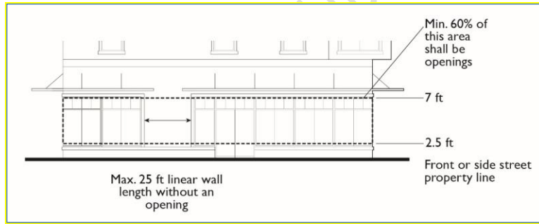
FIGURE 7-9-45.6. REQUIRED OPENINGS FOR NON-RESIDENTIAL USES
