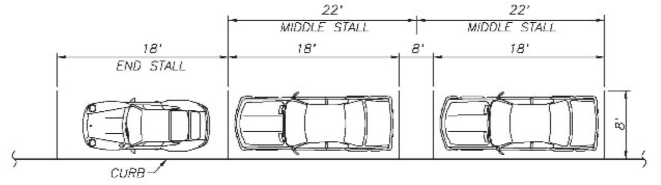
PARKING STALL DIMENSION PER ORANGE COUNTY STANDARDS, SECTION 7-9-145.4 (2X2) STALL LINES WILL BE MARKED AS SHOWN. ON-STREET TYPICAL PARALLEL PARKING STALL DETAIL N.T.S.
