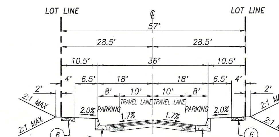
SECTION A-A "TOPAZ STREET" EXISTING INTERIOR STREET PUBLIC
