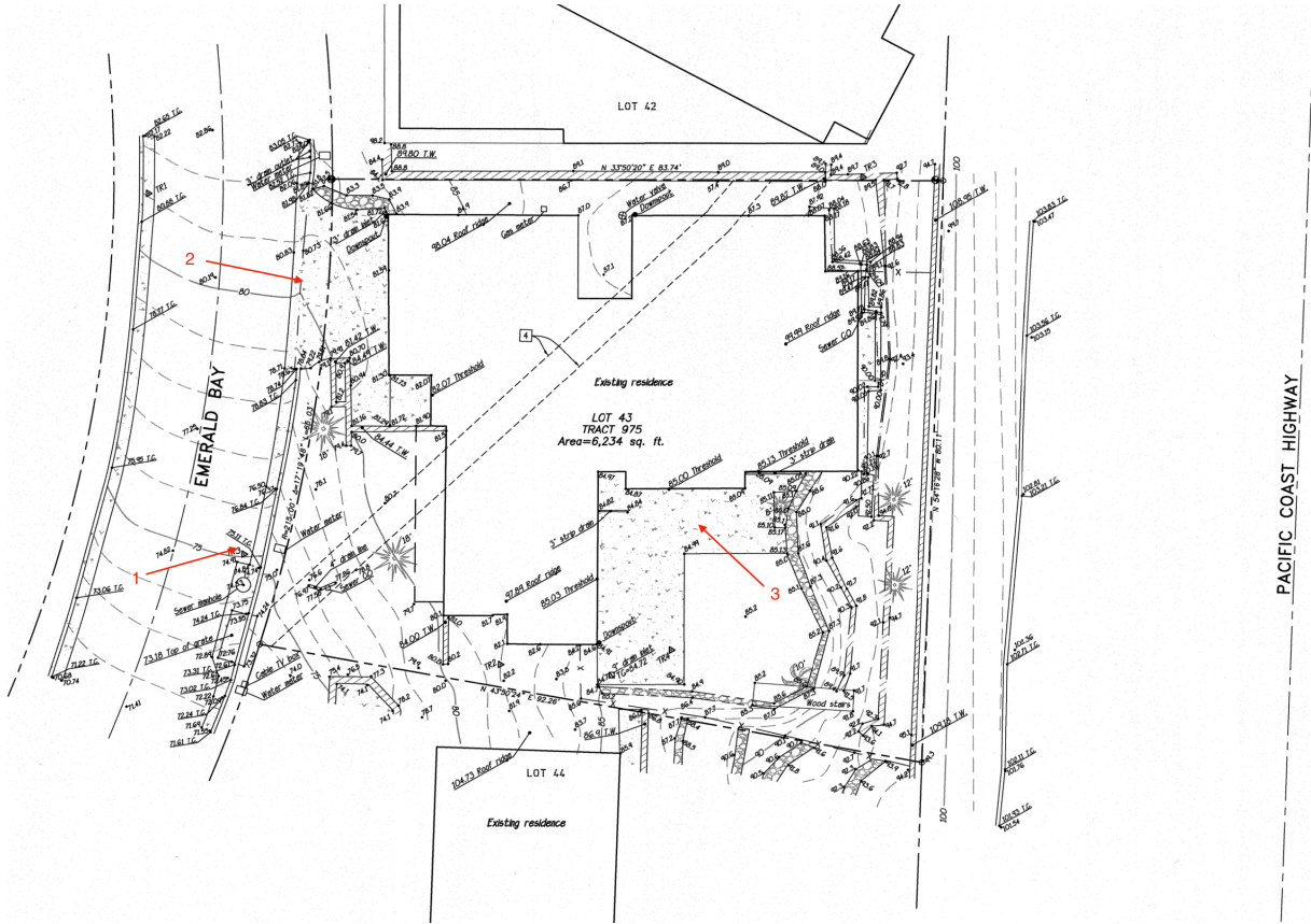
Site Photo Key Map
