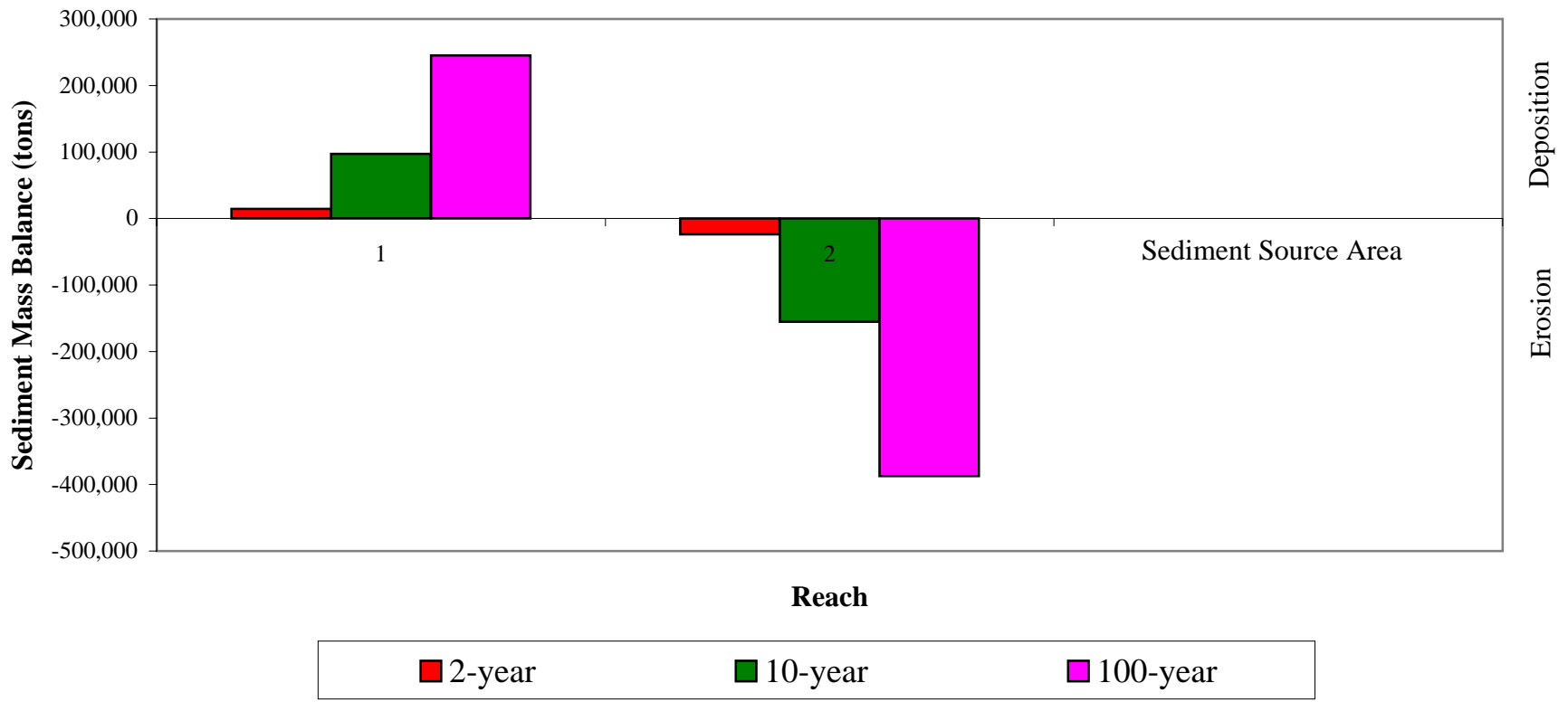
figure 4-8 Lucas Canyon Sub-basin Sediment Mass Balance
