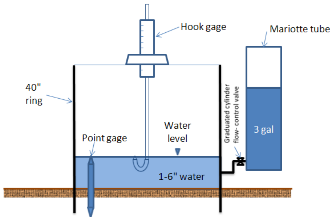
Figure VII.3. Single Ring Infiltrrometer Setup with Mariotte Tube
