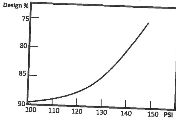
2 3 TABLE 903.3.5.3 4 Hydraulically Calculated Systems
